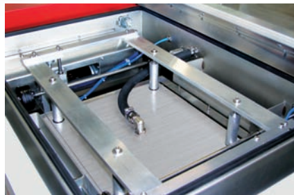
Evacuation unit
